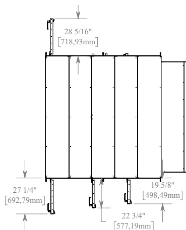
Dessus/Top
